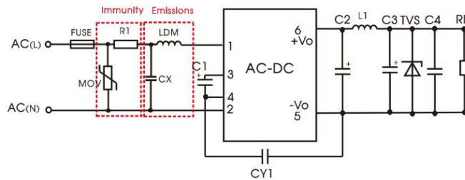
Recommended circuit 3
