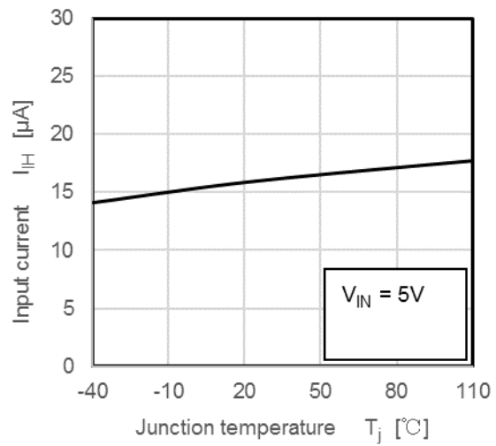
I_{IH} - T_j
